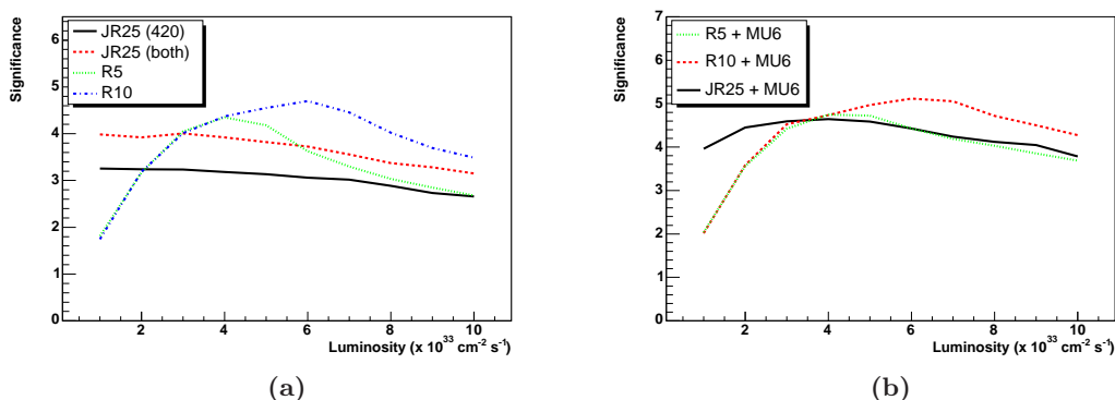
Figure 5. (a) Expected significance ( m_H = 120 GeV, c_H = 0.5 ) for the R5, R10 and JR25 triggers as a function of luminosity given three years of data acquisition at each luminosity. We assume that 10\text{fb}^{-1} of data is collected each year per 10^{33}\text{ cm}^{-2}\text{ s}^{-1} of luminosity, i.e. 120\text{fb}^{-1} of data is collected at 4 \times 10^{33}\text{ cm}^{-2}\text{ s}^{-1} . (b) The significance of the R5, R10 and JR25 triggers when combined with the MU6 trigger.
