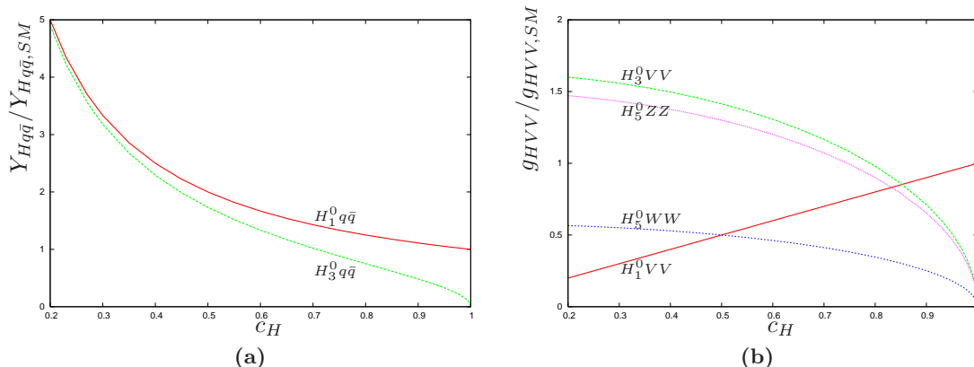
Figure 2. Couplings of the Higgs bosons to fermions (a) and gauge bosons (b), normalized by the Standard Model couplings.
